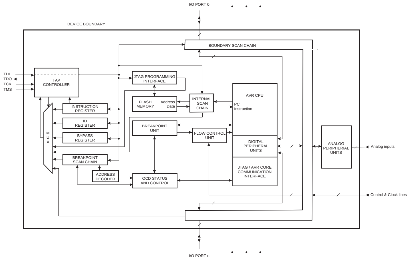
Figure 22-1. Block Diagram
