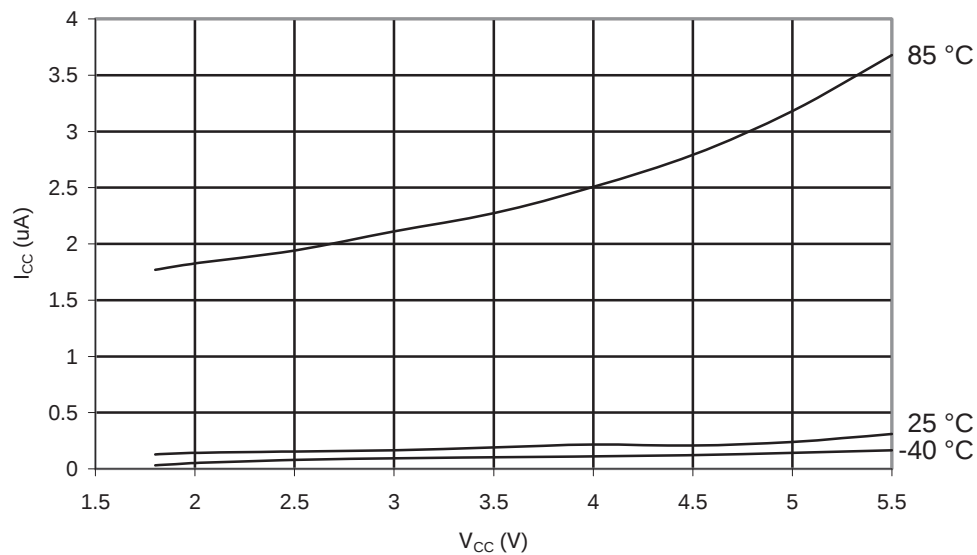
Figure 27-12. ATmega1284P: Power-down Supply Current vs. V_{CC} (Watchdog Timer Enabled)
