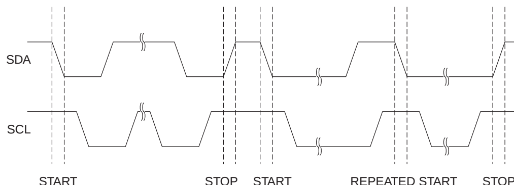
Figure 19-3. START, REPEATED START and STOP conditions
