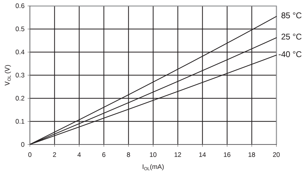
Figure 27-23. ATmega1284P: I/O Pin Output Voltage vs. Sink Current ( V_{CC} = 5V ).
